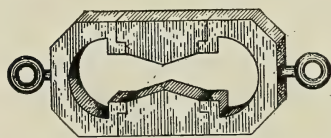
Courtesy of Humboldt Mfg. Co. FIG. 166.—Dow Ductility Mould.
